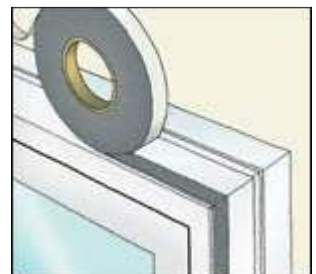
EXP6 Expanding Foam Tape can advantageously be mounted immediately prior to window installation.
