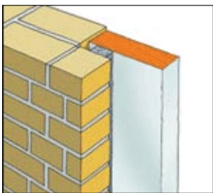
EXP6 Expanding Foam Tape renders a wind and water resistant sealing and in normal circumstances requires neither preparation nor finishing of the joint.
